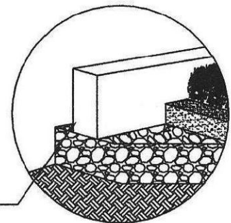
EDGE DETAIL- LANDSCAPE EDGING MATERIAL
