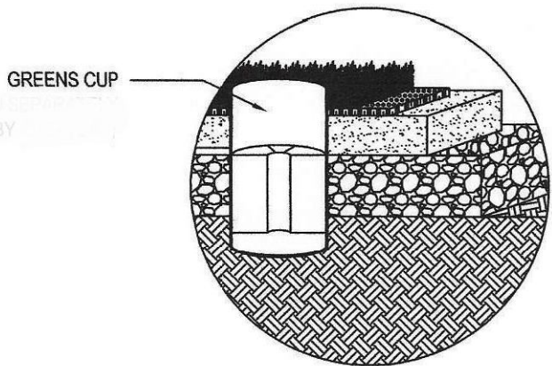
EDGE DETAIL- GREENS CUP
